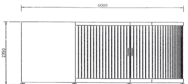
L=6 m. ALZADO FRONTAL CERRADO / SIDE VIEW CLOSED
