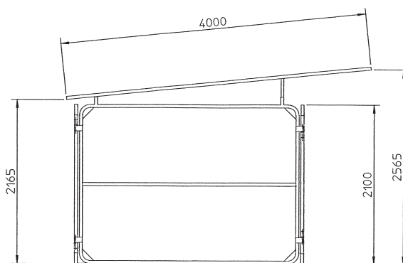
VISTA LATERAL SIDE VIEW
